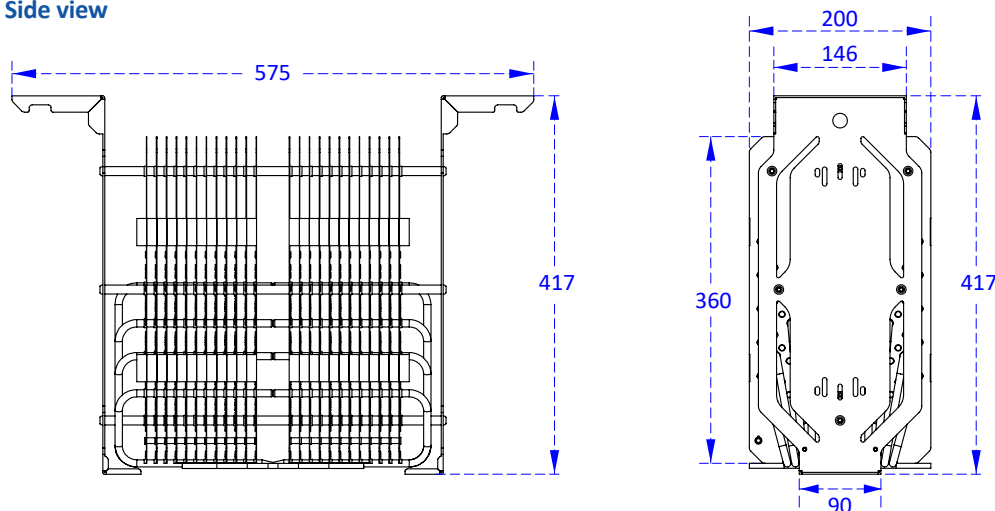
Side view
